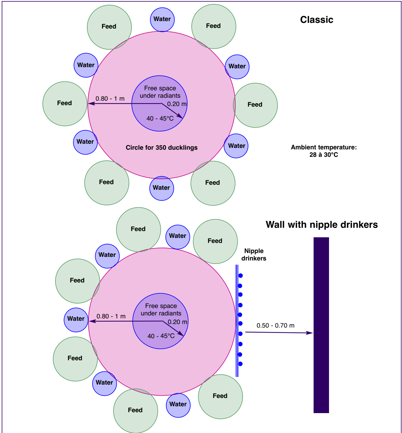
Fig.84.6. Brooding installation diagram: classic or with nipple drinkers (according to document Grimaud Frères)
