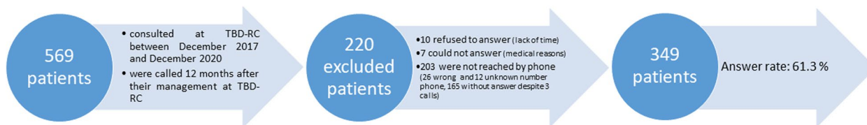
Fig. 2 Flow chart of the patients who were solicited to answer the satisfaction questionnaire at 12 months
